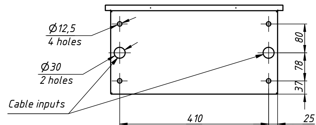
Instalation tamplate
