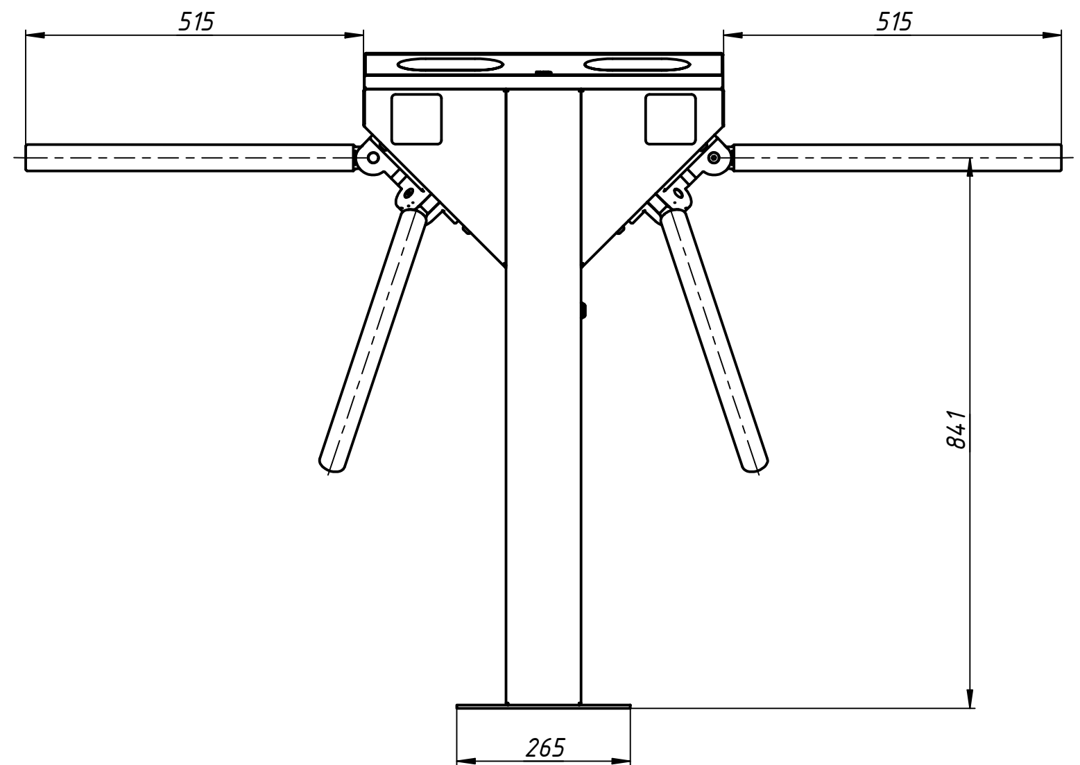
Instalation tamplate
